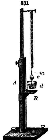
Spring or Jolly Balance for Specific Gravity
